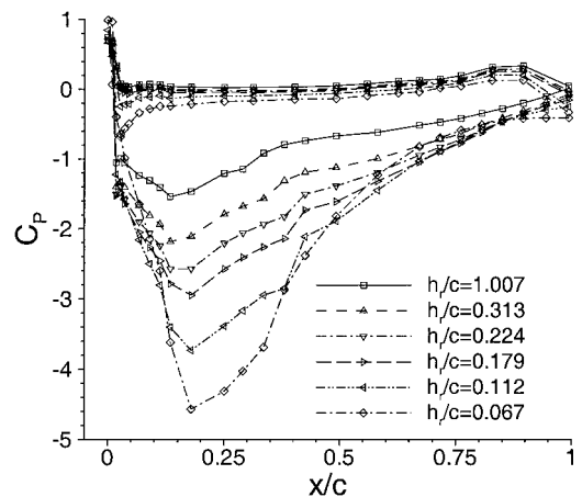
Fig. 6 Surface pressure distributions in ground effect at \alpha = 1 deg, transition-free.
