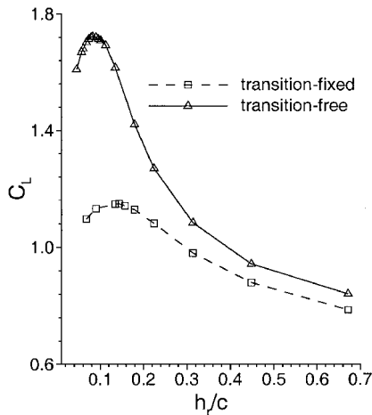
Fig. 11 Force coefficients in ground effect at \alpha = 1 deg; effect of transition fixing.
