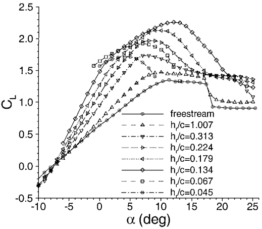
Fig. 9 Lift curves in ground effect, transition-free.
