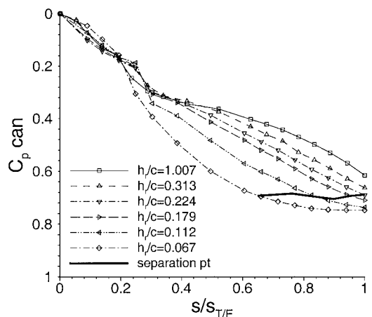
Fig. 7 Suction surface canonical-pressure recoveries in ground effect, transition-free at \alpha = 1 deg.
