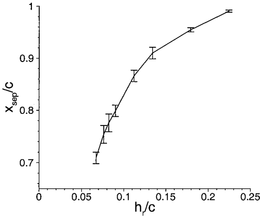
Fig. 5 Separation position with ride height at \alpha = 1 deg, transition-free.
