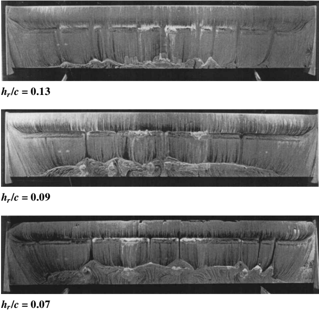
Fig. 4 Surface flow visualization at \alpha = 1 deg, transition-free.
