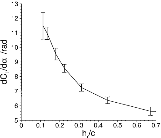
Fig. 10 Lift slope in moving ground effect, transition-free.
