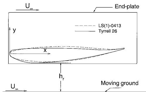
Fig. 1 Side view of Tyrrell-26 wing model with end plates at ride height h_r .
