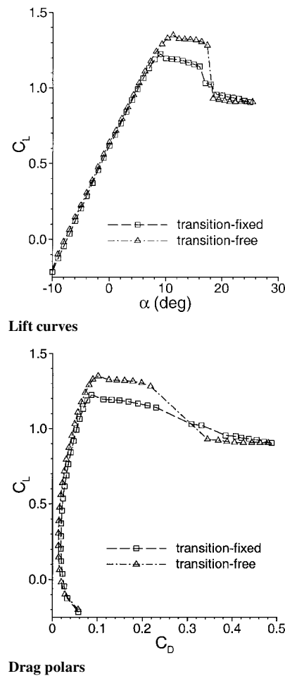
Fig. 2 Force coefficients in freestream.
