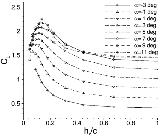
Fig. 8 C_L in ground effect, transition-free.
