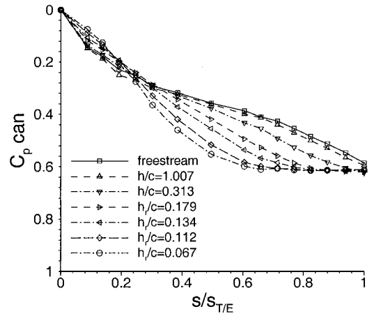
Fig. 13 Suction surface canonical recoveries in moving ground effect at \alpha = 1 deg, transition fixing.
