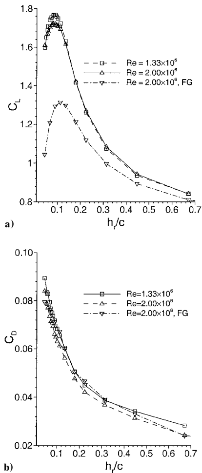
Fig. 3 Force coefficients in ground effect at \alpha = 1 deg, transition-free.
