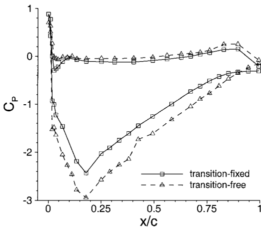
Fig. 12 C_p distributions in ground effect at h_r/c = 0.179 and \alpha = 1 deg; effect of transition fixing.
